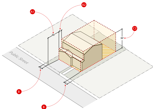
Figure 10 Illustrative Sloped Roof Building at Existing 0.6 FAR
