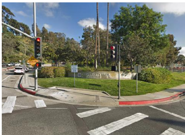
Not recommended: diagonal curb ramp configuration at Jefferson Boulevard and Duquesne Avenue. Source: Google Streetview
